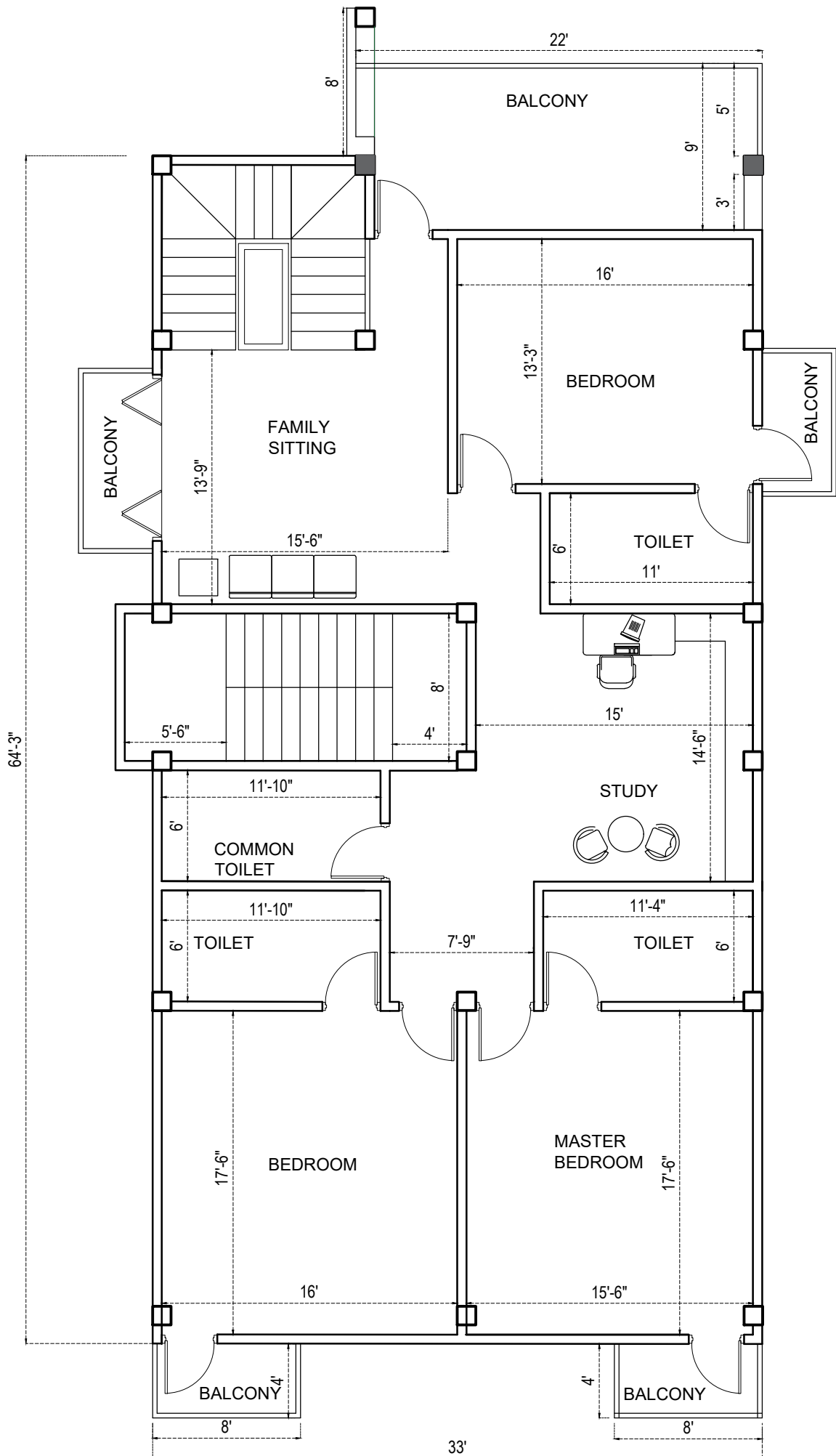
FIRST FLOOR PLAN 2480 SQFT
