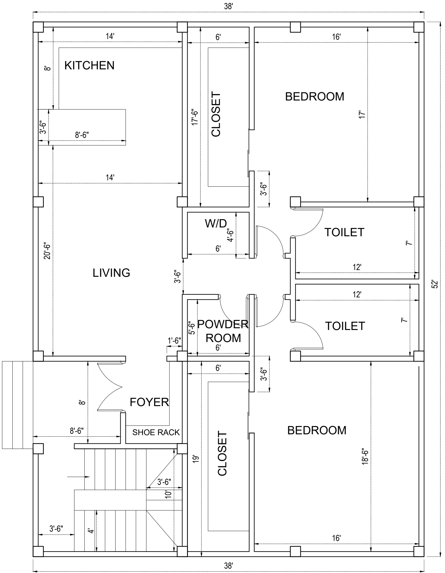
FLOOR PLAN
